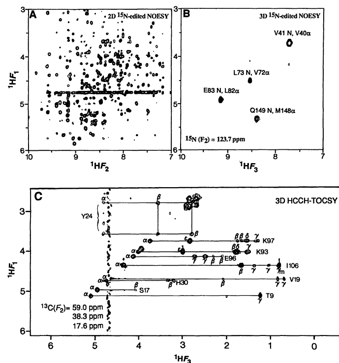
Fig. 5. Example of 2D and 3D spectra of IL-1 \beta recorded at 600 MHz (38, 43). The 2D spectrum in (A) shows the NH( F_2 axis)- \text{C}\alpha\text{H} ( F_1 axis) region of a 2D ^{15}\text{N} -edited NOESY spectrum. The same region of a single NH( F_3 )- ^1\text{H}(F_1) plane of the 3D ^{15}\text{N} -edited NOESY at \delta^{15}\text{N}(F_2) = 123.7 ppm is shown in (B). The actual 3D spectrum comprises 64 such planes and projection of these on a single plane would yield the same spectrum as in (A). In (C) a single ^1\text{H}(F_3) - ^1\text{H}(F_1) plane of the 3D HCCH-TOCSY spectrum at \delta^{13}\text{C}(F_2) = 38.3 \pm \text{nSW} (where SW is the spectral width of 20.71 ppm in the ^{13}\text{C} dimension) illustrates both direct and relayed connectivities originating from the \text{C}\alpha\text{H} protons. It is easy to delineate complete spin systems of long side chains such as Lys (that is, cross peaks to the \text{C}\beta\text{H} , \text{C}\gamma\text{H} , \text{C}\delta\text{H} , and \text{C}\epsilon\text{H} protons are observed) because magnetization along the side chain is transferred through large ^1J_{\text{CC}} couplings. Several features of the HCCH-TOCSY spectrum should be pointed out. First, extensive folding is used that does not obscure analysis as ^{13}\text{C} chemical shifts for different carbon types are located in characteristic regions of the ^{13}\text{C} spectrum with little overlap (41–43). Second, the spectrum is edited according to the chemical shift of the heteronucleus attached to the originating proton rather than the destination one. Third, multiple cross checks on the assignments are readily made by looking for the symmetry-related peaks in the planes corresponding to the ^{13}\text{C} chemical shifts of the destination protons in the original slice.
