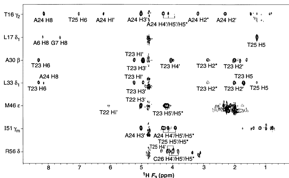
Fig. 2. Composite of ^{13}\text{C} -H strips taken from the 120-ms 3D ^{13}\text{C}(F_2) -separated, ^{12}\text{C} -filtered NOESY spectrum of the complex of the cGATA-1 DNA binding domain with DNA specifically illustrating NOEs between protons of the DNA (attached to ^{13}\text{C} along the F_3 axis) and protons of the peptide (attached to ^{13}\text{C} ). The ^1\text{H}(F_1)/^{13}\text{C}(F_2) shifts of T16 \gamma_2 , L17 \delta_1 , A30 \beta , L33 \delta_1 , M46 \epsilon , I51 \gamma_m , and R56 \delta are 1.40/23.07, 0.75/26.57, 1.74/18.74, 0.79/28.60, 2.25/17.11, 0.88/17.58, and 3.24/42.56 ppm, respectively.
