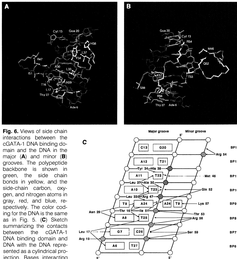
Fig. 6. Views of side chain interactions between the cGATA-1 DNA binding domain and the DNA in the major (A) and minor (B) grooves. The polypeptide backbone is shown in green, the side chain bonds in yellow, and the side-chain carbon, oxygen, and nitrogen atoms in gray, red, and blue, respectively. The color coding for the DNA is the same as in Fig. 5. (C) Sketch summarizing the contacts between the cGATA-1 DNA binding domain and DNA with the DNA represented as a cylindrical projection. Bases interacting with the protein are shaded; phosphates are represented as circles; circles with hatches directed toward the right and left indicate sites of interactions with sugar or phosphate or both in the major and minor grooves, respectively. The models in (A) and (B) were generated with the program VISP (52).
