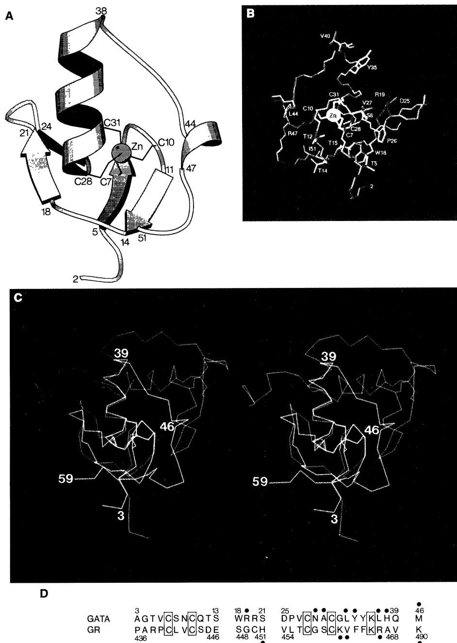
Fig. 4. (A) Schematic ribbon drawing of the core of the cGATA-1 DNA binding domain (residues 2 to 51). (B) Backbone (N, C \alpha , and C) trace (violet) of the core of the cGATA-1 DNA binding domain together with the zinc atom and side chains that are important for maintaining its structural stability (zinc, white; Cys, yellow; hydrophilic residues, orange; hydrophobic residues, green; and positively and negatively charged polar residues, blue and red, respectively). (C) Superposition of the C \alpha atoms of the cGATA-1 (green) and GR (red) DNA binding domains (the zinc and coordinating cysteine side chains are shown in yellow for cGATA-1 and in purple for the glucocorticoid receptor). (D) Sequence alignment of the cGATA-1 (2) and GR (14) DNA binding domains based on the structural alignment shown in (C). (The closed circles indicate residues that interact with DNA.) The GR sequence shown in (C) is that of the x-ray structure (14); residues 436 to 439 of the natural sequence, however, are PPKL. The programs Molscript (51) and VISP (52) were used to generate (A) and (B), respectively. The superposition and structural alignment in (C) was carried out with the program O (53).
