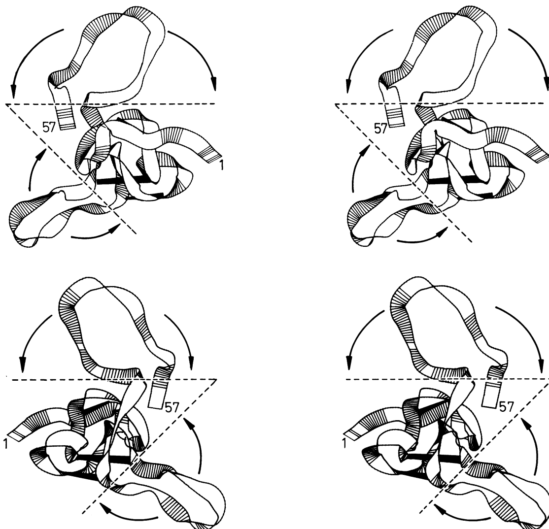
Fig. 5. Two stereoviews of the backbone atoms of the structure (\overline{\text{RDDG}})\text{m} represented as ribbon drawings illustrating the three domains of hirudin. The orientation of the two minor domains relative to the central core cannot be determined as no long range ( |i-j| > 5 ) interdomain NOEs could be observed (cf. Figure 1b). As a result the individual RDDG structures exhibit large displacements in the positions of the two minor domains relative to the central one (cf. Figure 1c and d) such that they can occupy any position indicated by the arrows within the boundaries defined by the dashed lines. These pictures were produced by a computer program written by Lesk and Hardman (1982).
